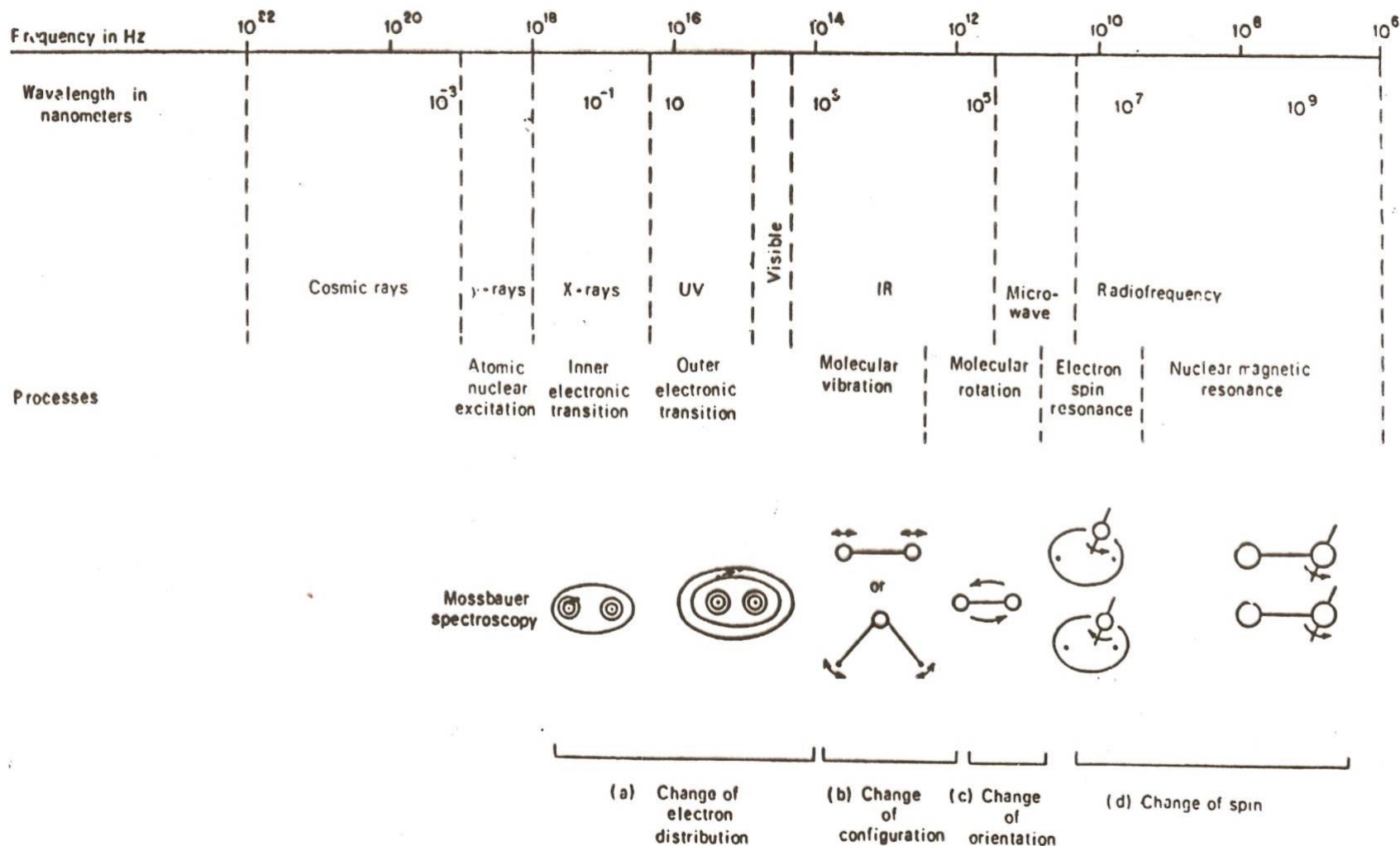
Figure 2.1 The complete spectrum of electromagnetic radiation, types of processes initiated and the corresponding spectroscopic terminology. (a) Change of electron distribution—x-ray, uv and visible electron spectroscopy; (b) change of configuration—vibration-rotation spectroscopy; (c) change of orientation-microwave spectroscopy; (d) change of spin—electron spin resonance (ESR) and nuclear magnetic resonance (NMR) spectroscopy.
