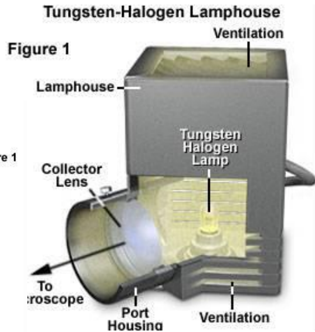
Modern Microscope Component Configuration
